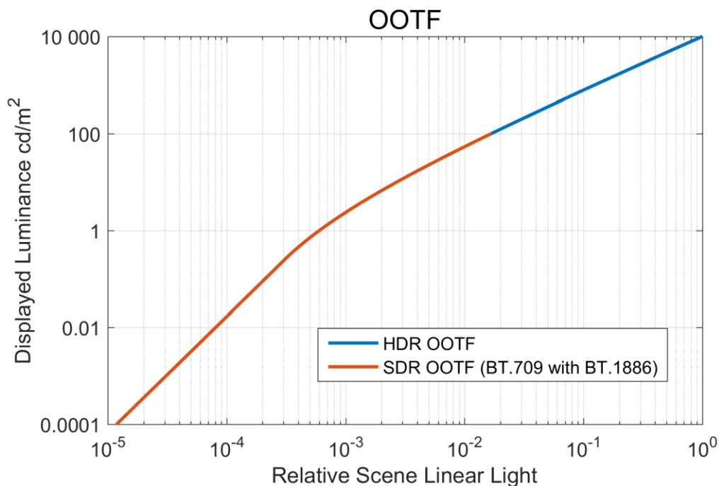
FIGURE 15 PQ and SDR OOTF
