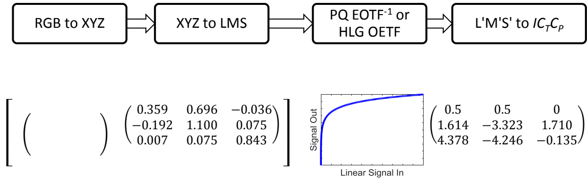
Camera RGB conversion to IC_{TC_P}
