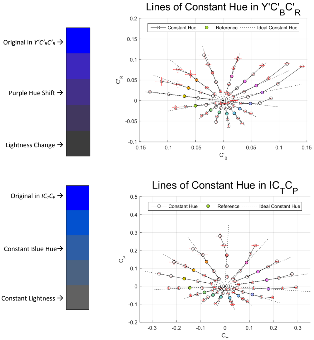
FIGURE 33 Blue Hue Linearity Comparison (using PQ)
