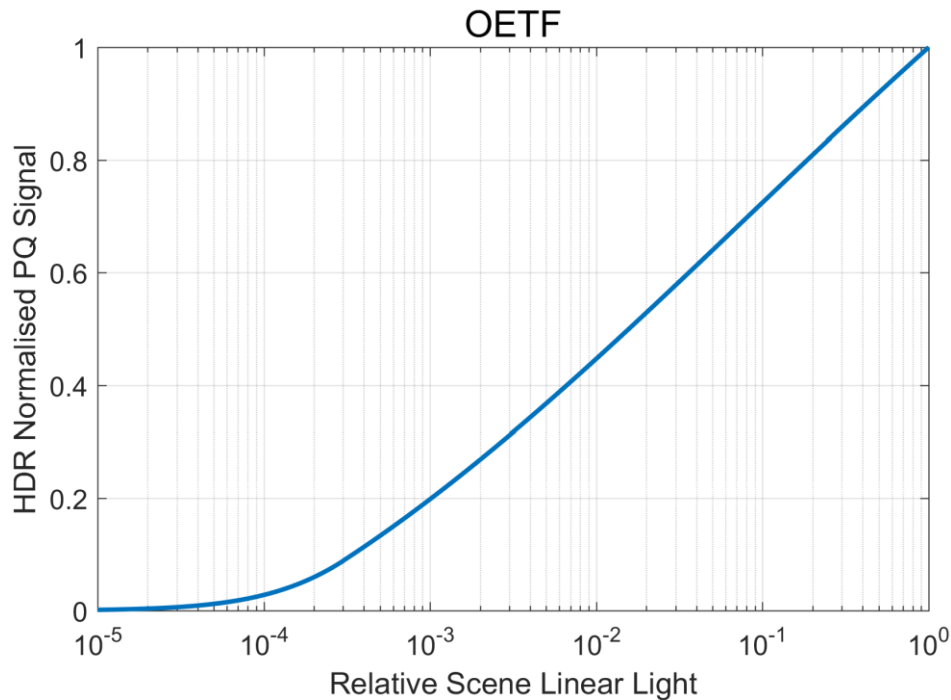
FIGURE 17 HDR OETF
