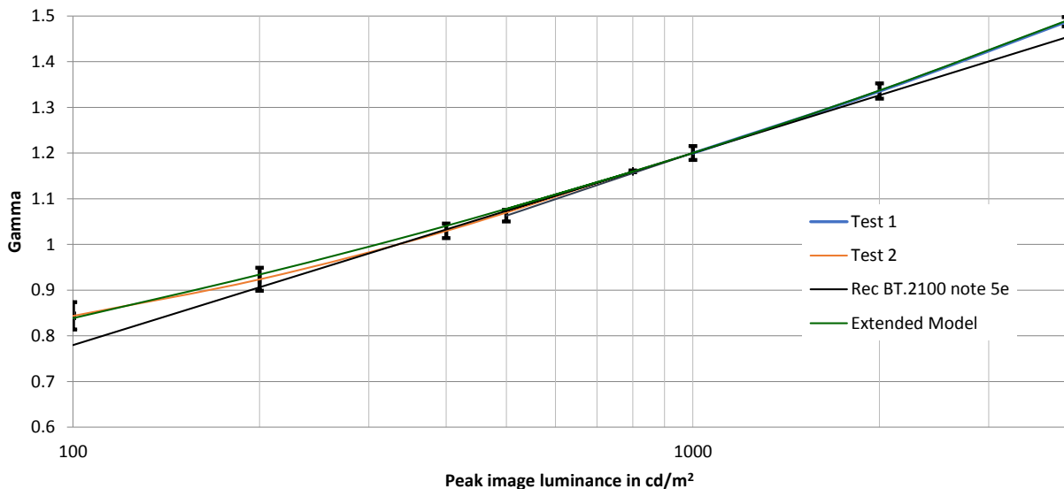
FIGURE 22 Gamma value to match images for different screen peak brightness
